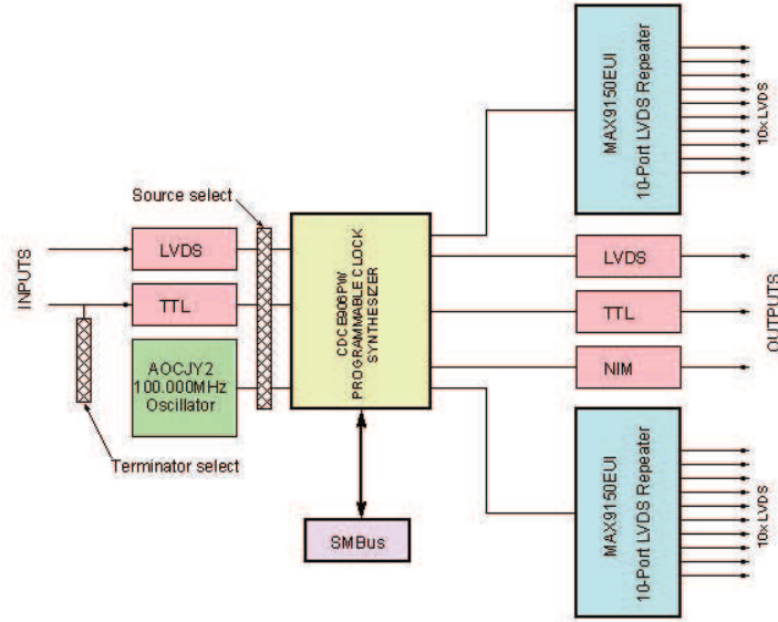
Figure 9. The block diagram of the CFM module
