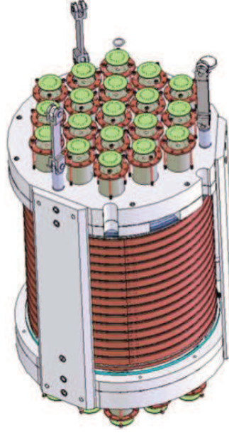
Figure 2. The DarkSide TPC showing the PMT and field shaping rings. The TPC is immersed in Lar but has a gas pocket just below the upper PMT window.
