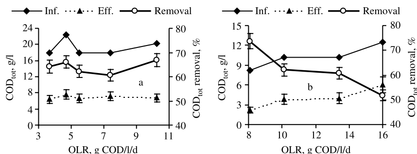
Figure 1 Influent and effluent total COD concentrations and total COD removal versus OLR under quasi-steady-state operation of UASB reactor treating the raw (a) and diluted (b) CM-1S
