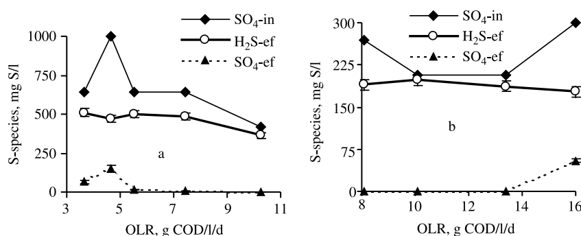
Figure 3 Influent and effluent sulphate as well as effluent sulphide concentrations versus OLR under quasi-steady-state operation of UASB reactor treating the raw (a) and diluted (b) CM-1S
