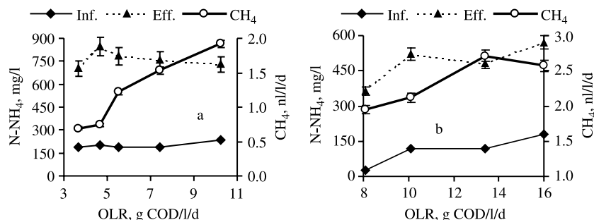
Figure 2 Influent and effluent ammonia concentrations and specific methane production versus OLR under quasi-steady-state operation of UASB reactor treating the raw (a) and diluted (b) CM-1S
