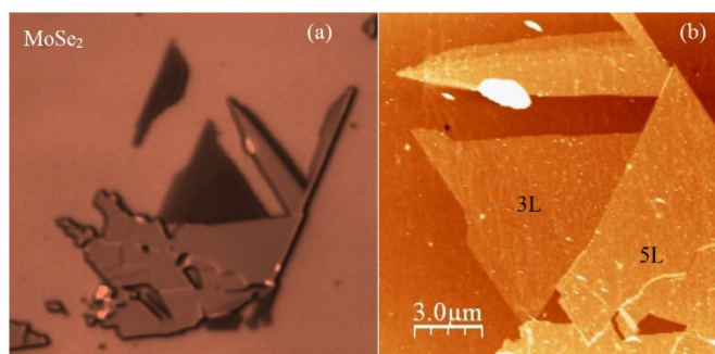
Figure 2. Optical and AFM images of MoS 2 nanolayers deposited on 270 nm SiO 2 with corresponding contrast and height.
