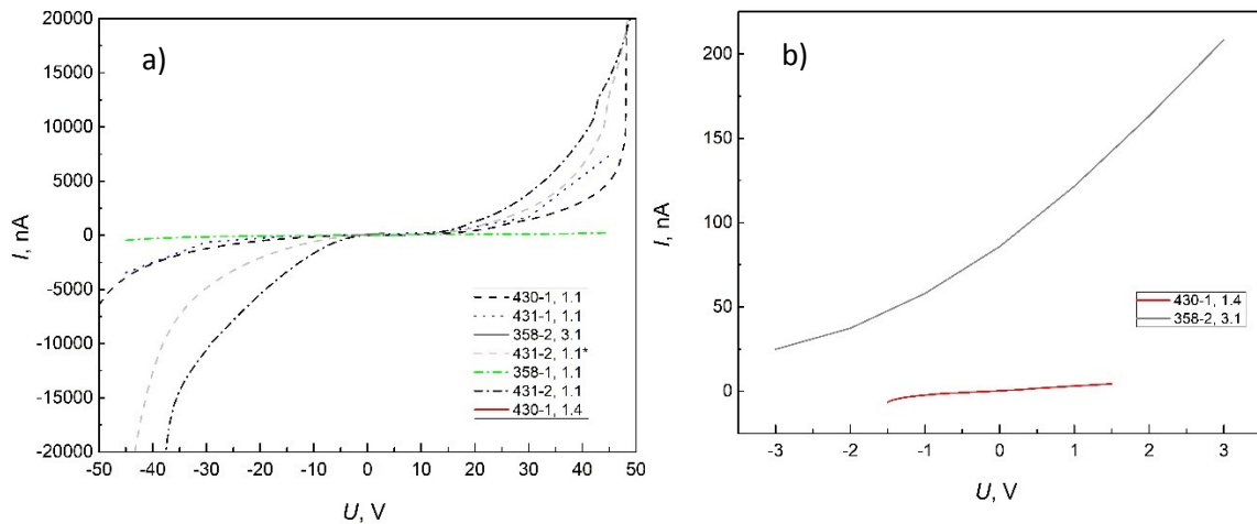
Figure 6. Dependence of dark current on the bias voltage of heterostructure LT-GaAs at room temperature with interdigitated contacts (a) and interdigitated contacts with closing of every second period by metal (b).
