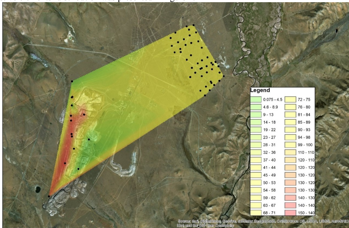
Fig.1. Distribution of absorbed dose rate in air from soil radioactive elements (nGy/h)
