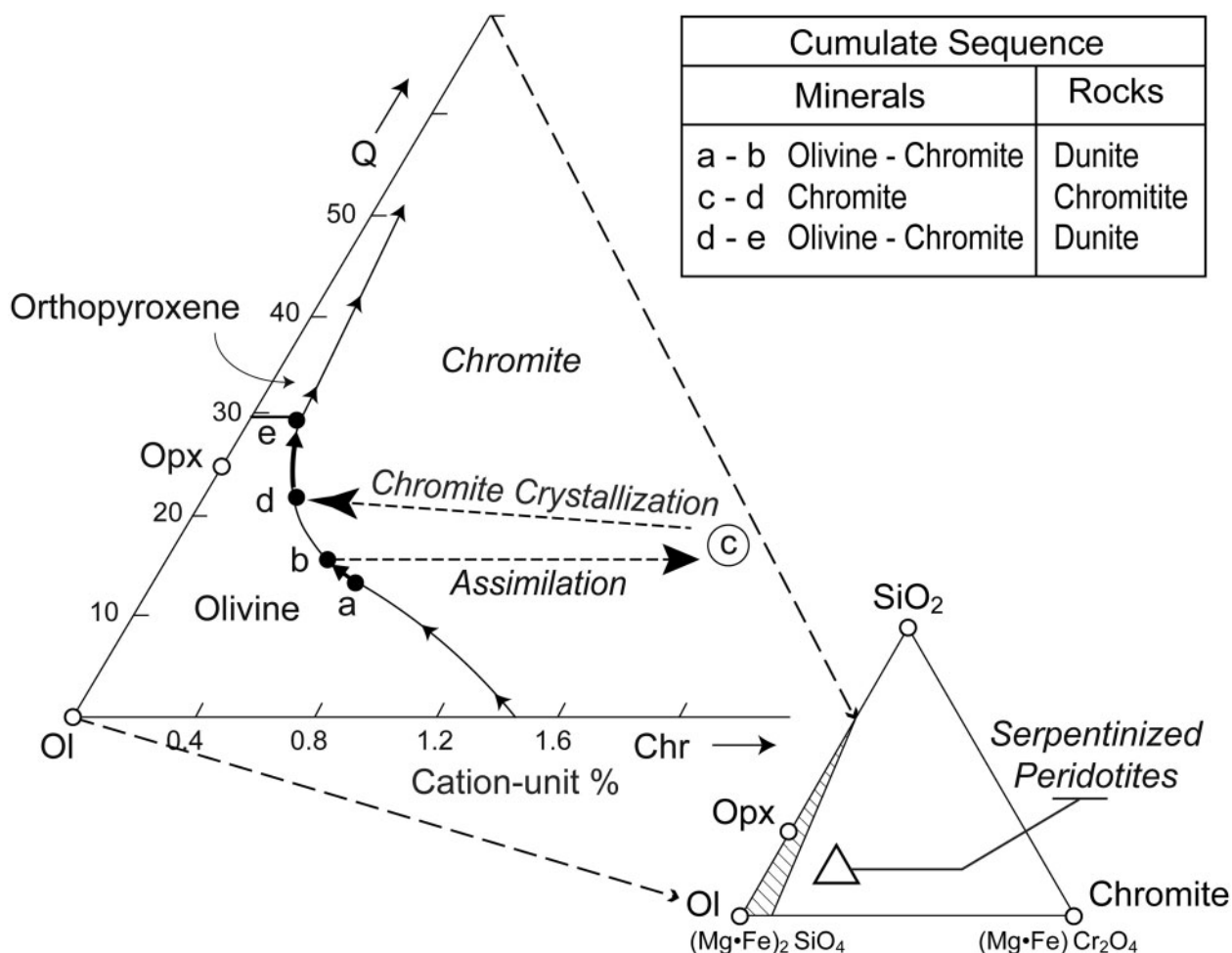
Fig. 7. Phase diagram model of Irvine (1975) applied to the petrogenetic model of the Maqсад MTZ chromitites formed through assimilation of a metamorphic mantle protolith by olivine-saturated MORB and fractional crystallization. The assimilation (b–c) is shown as a distinct process from the crystallization (a–b, c–d, and d–e). In reality, however, chromite could crystallize while the metamorphic protolith was being continuously assimilated. The composition of the serpentinized harzburgites corresponds to those of Li & Lee (2006).
