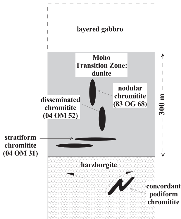
Fig. 2. Schematic geological cross-section of the Moho Transition Zone (MTZ) in the Maqad area of the Oman ophiolite. Chromitite ore bodies are localized in the host dunite layer (~300 m thickness).
