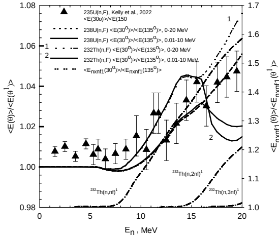
Fig. 2. ^{232}\text{Th}(n,F) and ^{238}\text{U}(n,F) ratios of \langle E \rangle, \langle E_{n,xnf} \rangle at 30^\circ/135^\circ
