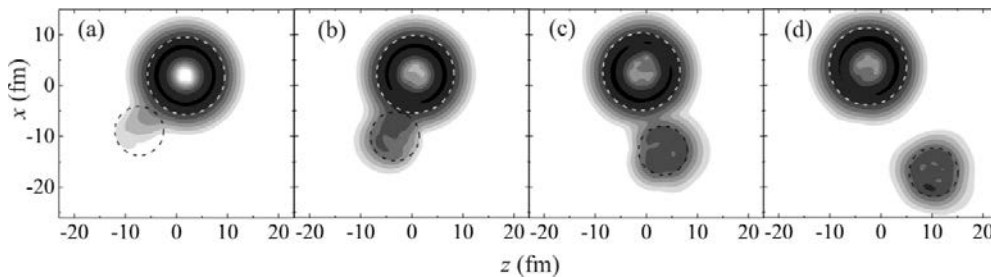
Fig. Example of time evolution of the probability density (shades of grey, logarithmic scale) for the proton of the 1h_{1/2} subshell of the ^{197}\text{Au} nucleus in the collision ^{48}\text{Ca} + ^{197}\text{Au} at an energy of 400 MeV in the center-of-mass frame and impact parameter 9 fm. The location of panels (a)–(d) corresponds to time
