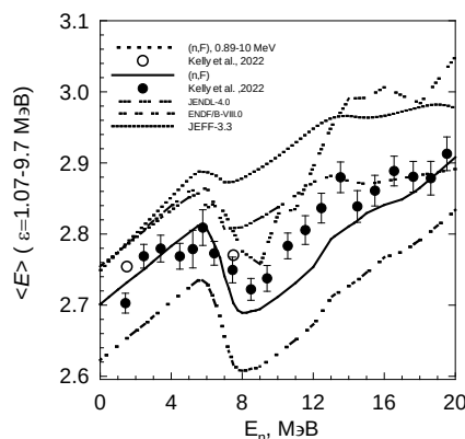
Рис. 2. \langle E \rangle ^{240}\text{Pu}(n,F)
