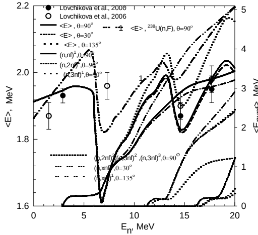
Fig. 1. \langle E \rangle and \langle E_{n,xnf} \rangle of ^{232}\text{Th}(n,F) and ^{238}\text{U}(n,F)
