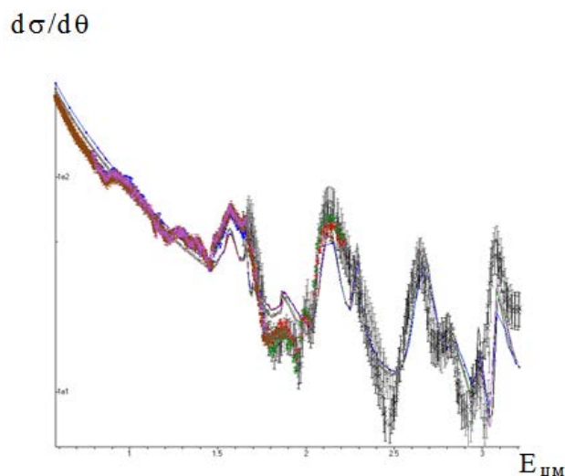
Figure. Excitation function of the ^{16}\text{O}(d,d_0) reaction at the angles of 153.6 – 169.2 degrees in the center-of-mass system (points – experimental data, solid curves – fitting results)
