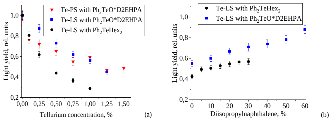
Light yield as a function of (a) tellurium concentration, (b) diisopropylnaphthalene concentration for tellurium-loaded organic scintillators (relative to the light yield of unloaded LS and PS)
