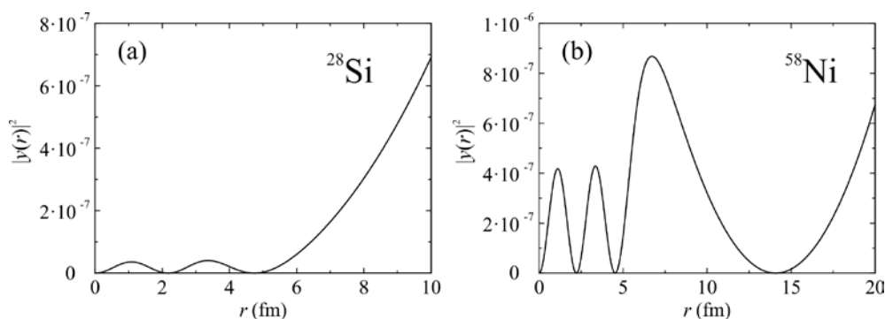
Fig. Radial probability densities for the s-states of slow neutrons upon elastic scattering on the ^{28}\text{Si} (a) and ^{58}\text{Ni} (b) nuclei
