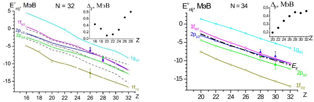
Neutron single-particle energies of isotones with N = 32 (left), 34 (right). In the insets, the differences \Delta_F = |E_F - \langle E_{2p_{3/2}}, E_{2p_{1/2}} \rangle| and \Delta_F = |E_F - \langle E_{2p_{1/2}}, E_{1f_{5/2}} \rangle| are shown for isotones with N = 32 and 34 respectively
