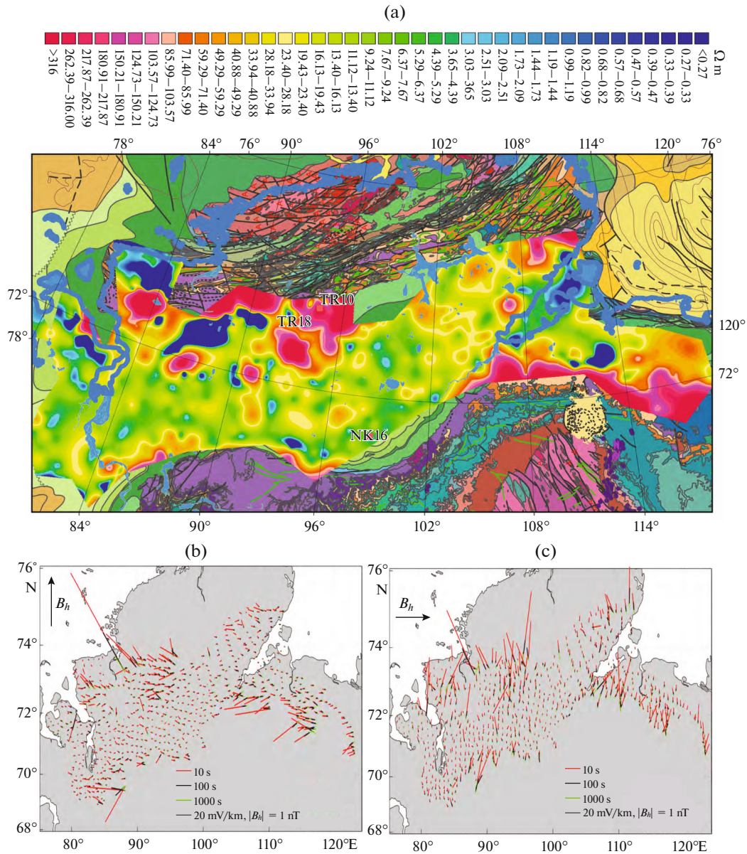
Fig. 4. Spatial distribution of effective apparent resistivity \rho_{\text{app}} over the YKRT area for T = 10 s according to the areal array of MT impedance estimates (Slinchuk et al., 2022) (a), and the impedance-based spatial distributions of vectors of the horizontal electric field E(x, y, T) , induced by the homogeneous harmonic geomagnetic field B_h(T) with an amplitude of 1 nT, geographically oriented N–S (b) and E–W (c), for the periods 10 s (red), 100 s (black), and 1000 s (green); a map of electrical conductivity averaged by the upper 10 km layer in the model (Alekseev et al., 2015) (d), and amplitude geoelectrical responses, calculated in the model, to excitation by the homogeneous harmonic geomagnetic field B_h(T) with a unit amplitude for the periods 10 s (e) and 100 s (f) (fragments of the maps built for the territory of the Russian Federation in (Kozyreva et al., 2022)).
