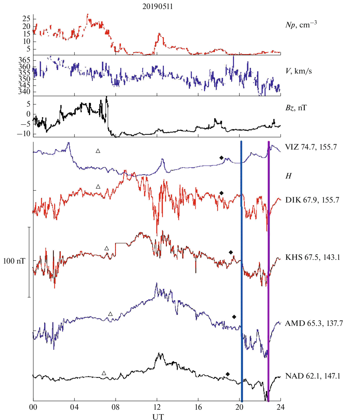
Fig. 5. Variations of the magnetic field H -component (towards geomagnetic north), recorded at VIZ, DIK, KHS, AMD, NAD (by 140^\circ – 150^\circ magnetic longitude profile, geomagnetic coordinates of stations in degrees), in the interval 00–24 UT on May 11, 2019. Three graphs on top: variations in the density ( Np ), velocity ( V ) of the solar wind and B_z —component of the interplanetary magnetic field. Triangle symbols indicate local midday, diamond symbols stand for midnight. The blue and pink vertical lines indicate the time points 20:08 UT and 22:43 UT, accordingly, for which Fig. 2 shows vectors of synthesized geoelectrical responses at NK16, TR18, TR08, TR10.
