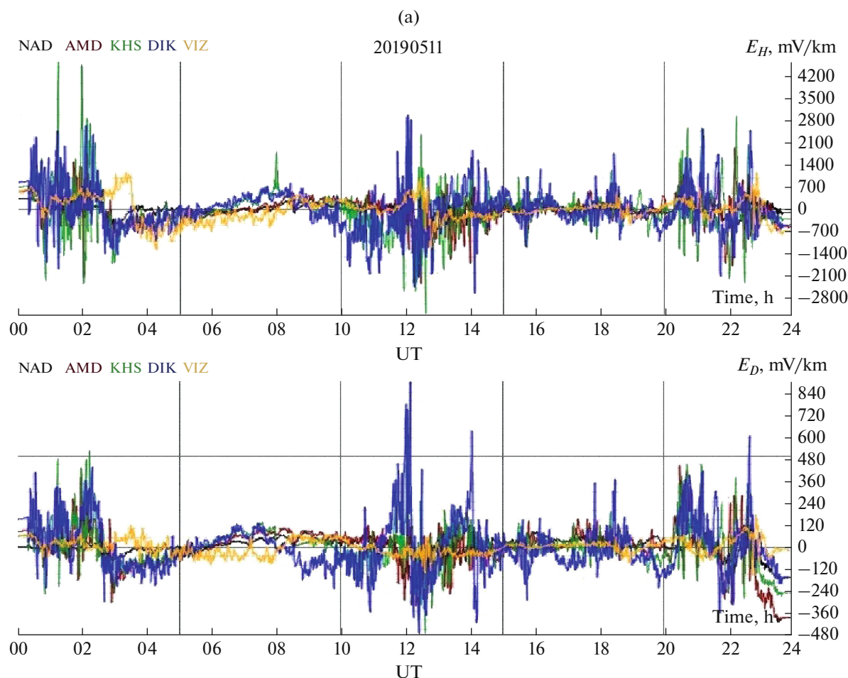
Fig. 7. Results of synthesis of time series of variations E_H , E_D electric field components by experimental frequency dependences Z(f) at the sounding locations TR10 (a) and NK16 (b) for the record of magnetic variations in the interval 00–24 UT on May 11, 2019 (Fig. 5) at the magnetic observation stations NAD, AMD, KHS, DIK, VIZ. Panel (c) shows time derivatives of variations of the components H and D (nT/s). Locations, frequency dependences Z(f) and the local geoelectrical setting are shown in Fig. 2, Fig. 3, and Fig. 4, respectively.
