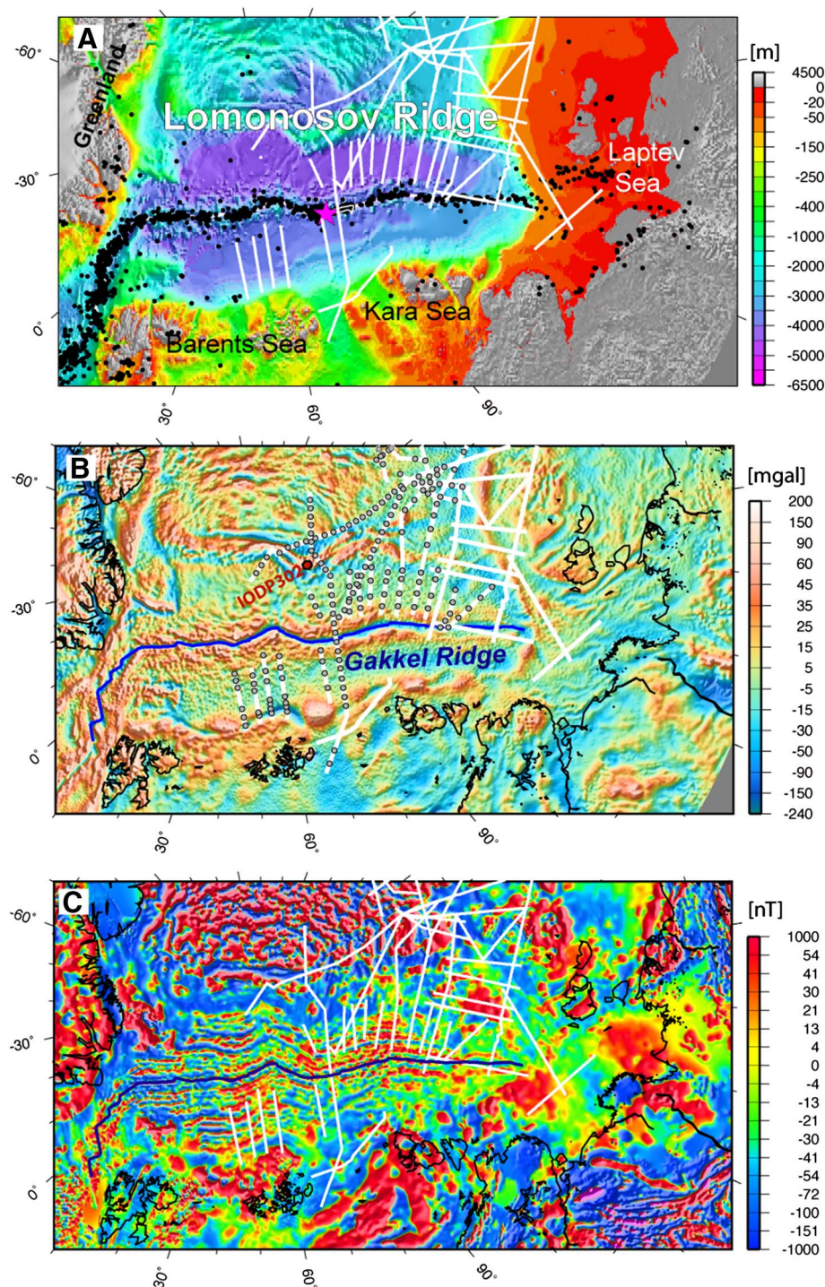
Fig. 2. Gridded geophysical data used in this study and location of Russian seismic profiles discussed in the text (in white): A. bathymetry (GEBCO2014/IBCAOV3); B. free air gravity anomalies (DTU13, Andersen et al., 2014); C. magnetic anomaly grid (CAMP-GM, Gaina et al., 2011). Gakkel Ridge location is from Engen et al. (2002). In panel A, black dots are earthquake locations from the ISC ( www.isc.ac.uk/iscbulletin ) and EMSC ( www.emsc-csem.org ) earthquake catalogues from 1960 to 2016. The latest large earthquake (magnitude 4.7) erupted on 22.10.2016 on the Gakkel Ridge is shown by the magenta star. Russian sonobuoy locations are shown as open circles (panel B). (For interpretation of the references to colour in this figure legend, the reader is referred to the web version of this article.)
