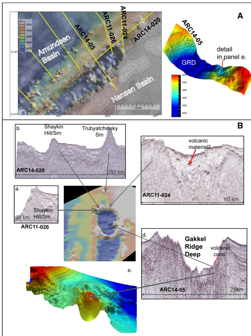
Fig. 12. The Gakkel Ridge Deep. A. Bathymetry (IBCAO v3, 500 m grid resolution) and contours from magnetic anomaly grid CAMP-GM (Gaina et al., 2011). Yellow lines are seismic profiles discussed in this study. B. 3D image of bathymetry (same as in A.), and detailed images of seismic data showing volcanic constructs within GRD and on its flanks. Panel e shows gridded multibeam data (90 m cell size) collected along ARC14-05 profile. (For interpretation of the references to colour in this figure legend, the reader is referred to the web version of this article.)
