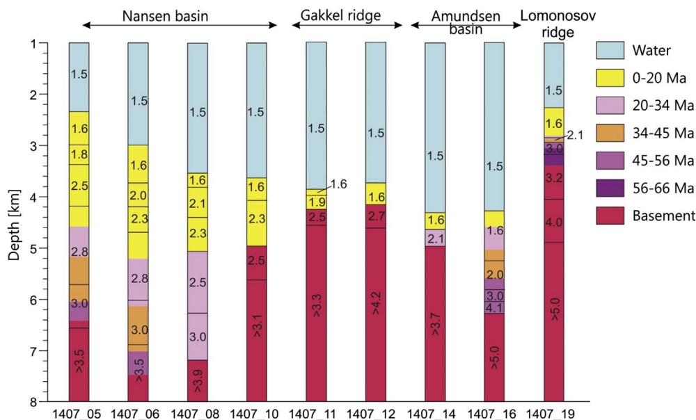
Fig. 4. Seismic velocity-depth model for the Nansen and Amundsen basins based on sonobuoy data recorded along profile ARC14-07 (see profile and sonobuoys location in Figs. 2 and 6).
