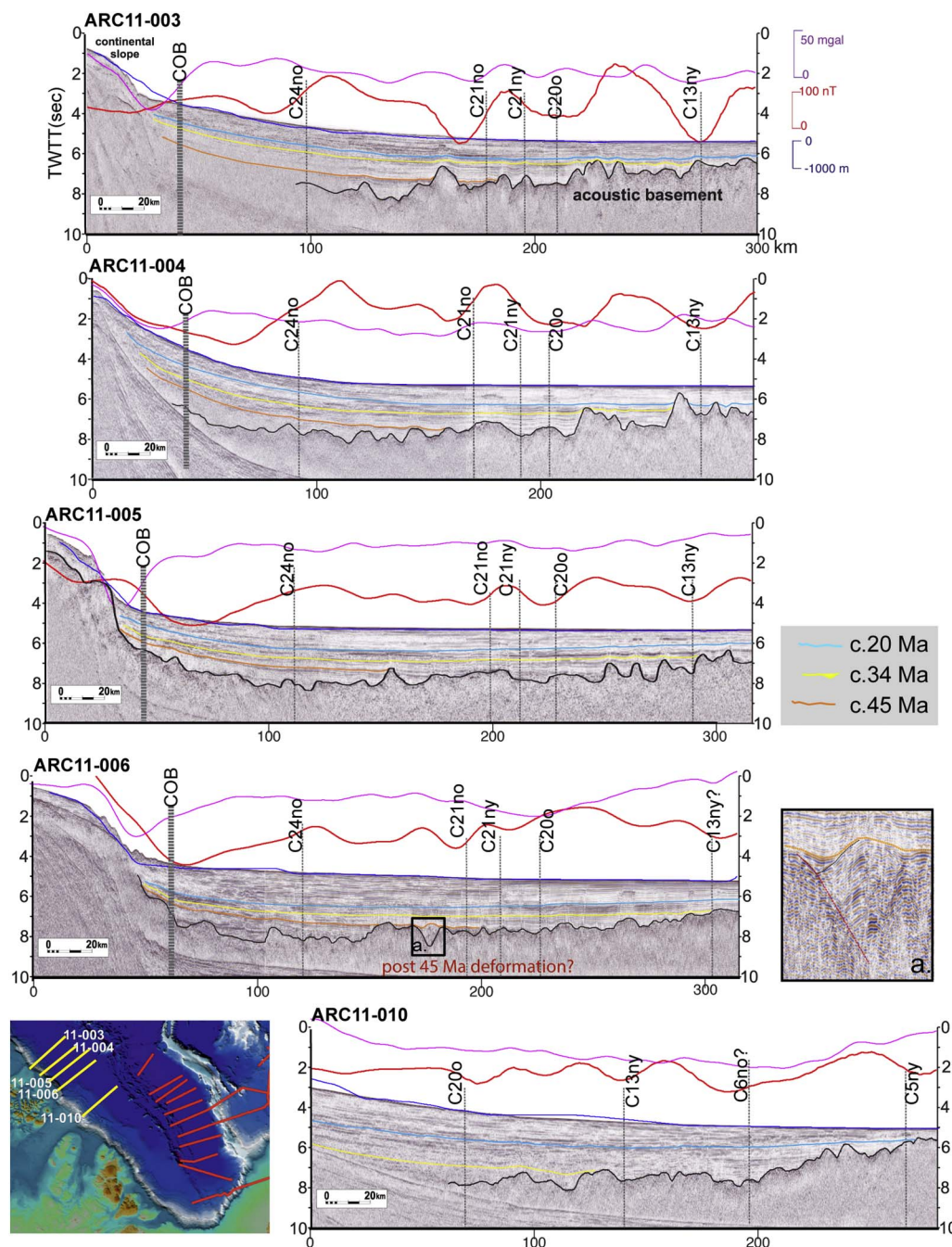
Fig. 5. Arktika-2011 (Nansen Basin) seismic profile interpretation (profile location shown in the left lower corner and in Fig. 1, un-interpreted data in Fig. S1). Magnetic anomalies (CAMP-GM, Gaina et al., 2011) along the same profiles are shown in red; free air gravity anomalies (DTU13, Andersen et al., 2014) - in magenta, and bathymetry (GEBCO2014/IBCAOV3) - in blue. “C” stands for magnetic chron. The interpreted age of seismic horizons is guided by the oceanic basement age and correlations with pan-Arctic geological and geophysical data. (For interpretation of the references to colour in this figure legend, the reader is referred to the web version of this article.)
