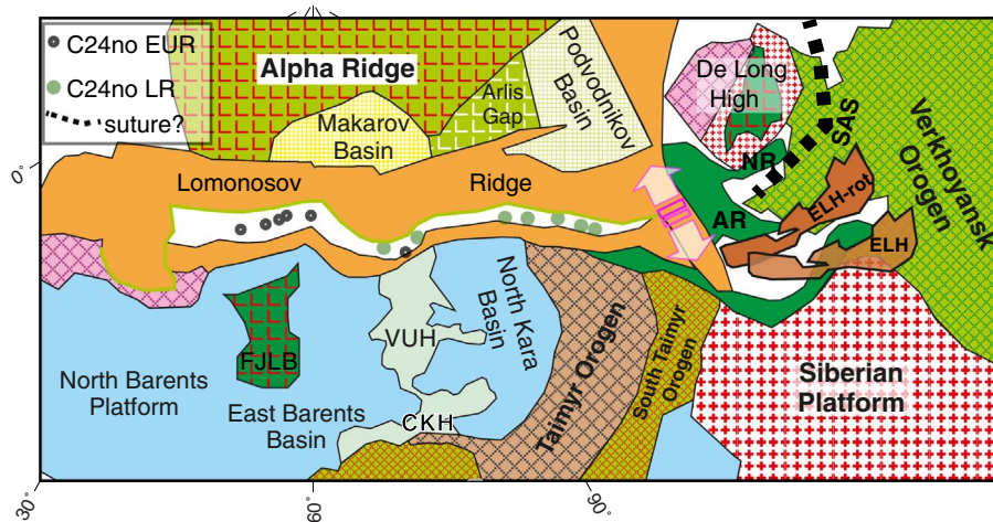
Fig. 13. Main tectonic provinces flanking Eurasia Basin (as in Fig. 3) reconstructed at C24no time (53.98 Ma). Barents/Kara seas and Lomonosov Ridge continental margin outlines have been adjusted according to the COB (continent-ocean boundary) interpretation shown in Figs. 5, 6, 8 and 9. Magnetic picks for C24no shown in green and grey. ELH is East Laptev Horst shown in two positions: semi-transparent polygon shows ELH location in the absence of Paleocene rifting in the East Laptev Sea rift system; the brown polygon shows the rotated ELH to account for rifting that may have occurred prior to Eurasia-North America break-up. Abbreviations: AR-Anisin Rift depocenter, CKH-Central Kara High, FJL-Franz Josef Land, NR-Novosibirsk rift depocenter, SAS-South Anyui Suture, VUH-Vize-Ushakov High. (For interpretation of the references to colour in this figure legend, the reader is referred to the web version of this article.)
