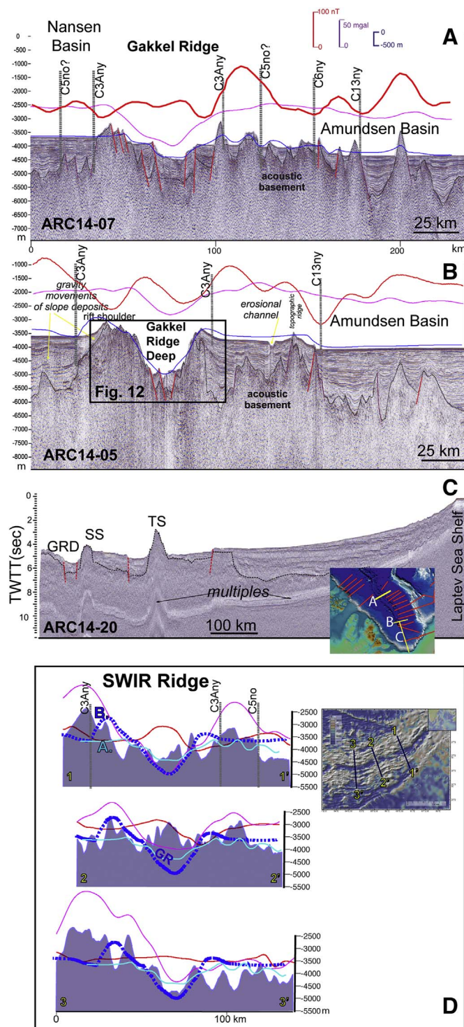
Fig. 11. Interpretation of seismic profiles across the Gakkel Rift valley, and comparison with selected Southwest Indian Ridge bathymetric profiles (location in inset figure and Fig. 1, un-interpreted data in Fig. S5). A is a fragment of seismic profile ARC 14-07 (see Fig. 5A), B is a fragment of seismic profile ARC 14-05 (Fig. 1), and C is seismic profile ARC 14-20. Red solid lines are possible normal faults. Abbreviations: GRD - Gakkel Ridge Deep, SC - Shaykin seamount, TS - Trubyutchinsky seamount. C. Bathymetry (GEBCO2014), magnetic anomalies (WDMAM) and free air gravity (DTU13, Andersen et al., 2014) along selected profiles across the Southwest Indian Ridge (SWIR); see profile location on the right hand side. Cyan profile and blue thick dotted line are segments of the Gakkel Ridge bathymetric profiles shown in panel A and B, respectively, plotted at the same scale with the SWIR bathymetry. (For interpretation of the references to colour in this figure legend, the reader is referred to the web version of this article.)
