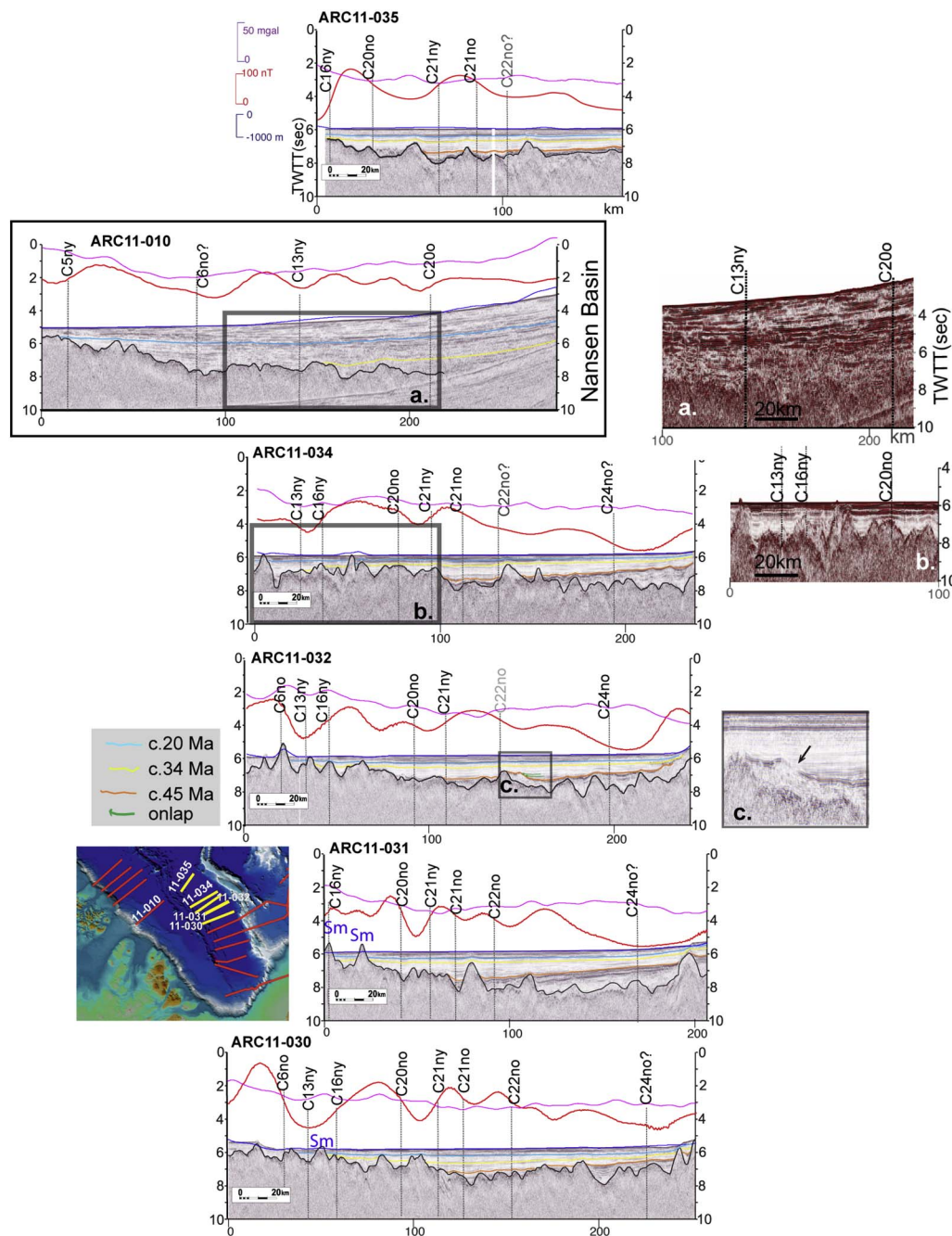
Fig. 8. Arktika-2011 (north Amundsen Basin) seismic profile interpretation (location in inset figure and Fig. 1, un-interpreted data in Fig. S3). Potential field data, bathymetric profiles, and chron interpretations as in Fig. 5. “Sm” stands for seamount.
