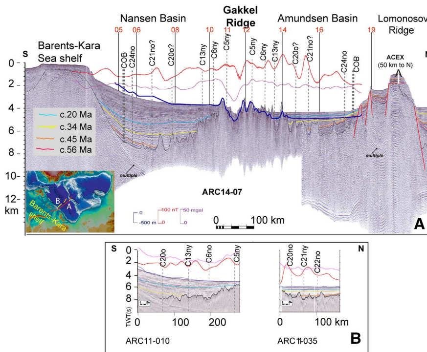
Fig. 6. A. Seismic line ARC14-07 across the entire Eurasian Basin and its continental margins (location in Fig. 1, un-interpreted data in Fig. S2), and B. Seismic lines ARC11-010 (Nansen Basin) and ARC11-035 (Amundsen Basin) showing incomplete Eurasia Basin conjugate flanks. Red numbers in panel A indicate the location of sonobuoy deployments. Potential field data, bathymetric profiles, and chron interpretations as in Fig. 5. (For interpretation of the references to colour in this figure legend, the reader is referred to the web version of this article.)
