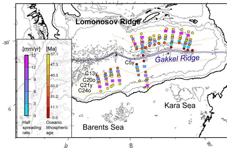
Fig. 10. Magnetic anomaly identifications and seafloor half spreading rates calculated according to the new oceanic lithosphere age identifications along the seismic profiles shown in Figs. 5, 6, 8 and 9 (see also Table 2).
