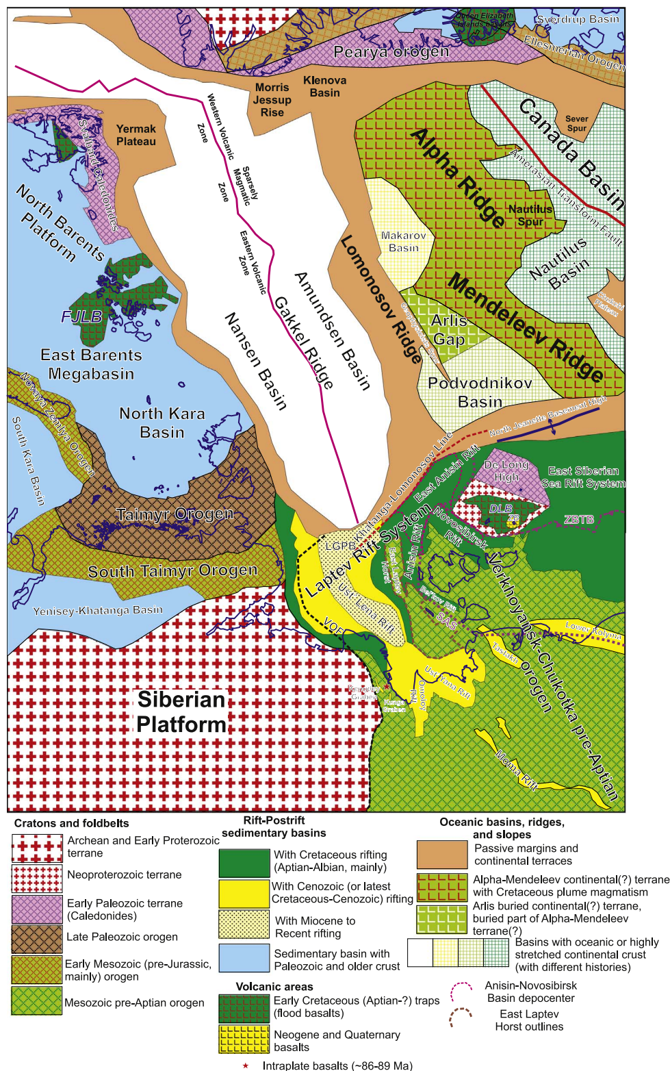
Fig. 3. High Arctic tectonic map revised after Nikishin et al. (2014, 2017). Abbreviations: DLB – De Long Basalts (128–112 Ma), LGPB – Laptev-Gakkel pull-apart basin (c. Oligocene to Recent), SAS – South Anyui Suture (c. 130–120 Ma), VOF – Verkhoyansk Orogen Front, ZB – Zhokhov Basalts (1–3.6 Ma), ZBTB – Zhokhov buried thrust belt.
