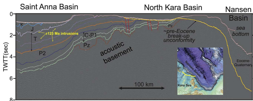
Fig. 7. Seismic profile PGS-GWL-006 interpretation along the Nansen Basin passive continental margin. The lower sedimentary cover may be Eocene strata deposited on acoustic basement and North Kara Basin Paleozoic sedimentary sequences. This indicates pre-Eocene uplift of the northern Kara margin. Profile location in inset figure and Fig. 1.
