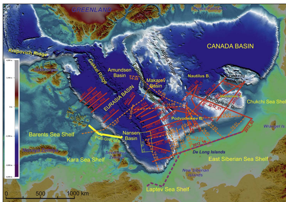
Fig. 1. Location and names of the new Russian Arctic seismic profiles used for the tectono-stratigraphic interpretation. Background map: Arctic topography and bathymetry (Jakobsson et al., 2012). Red lines are Russian Federal projects Arktika-2011 and Arktika-2012 seismic profiles, orange lines – Arktika-2014 seismic profiles, yellow line – “Geology Without Limits” selected profiles, purple lines – ION selected seismic profiles. (For interpretation of the references to colour in this figure legend, the reader is referred to the web version of this article.)
