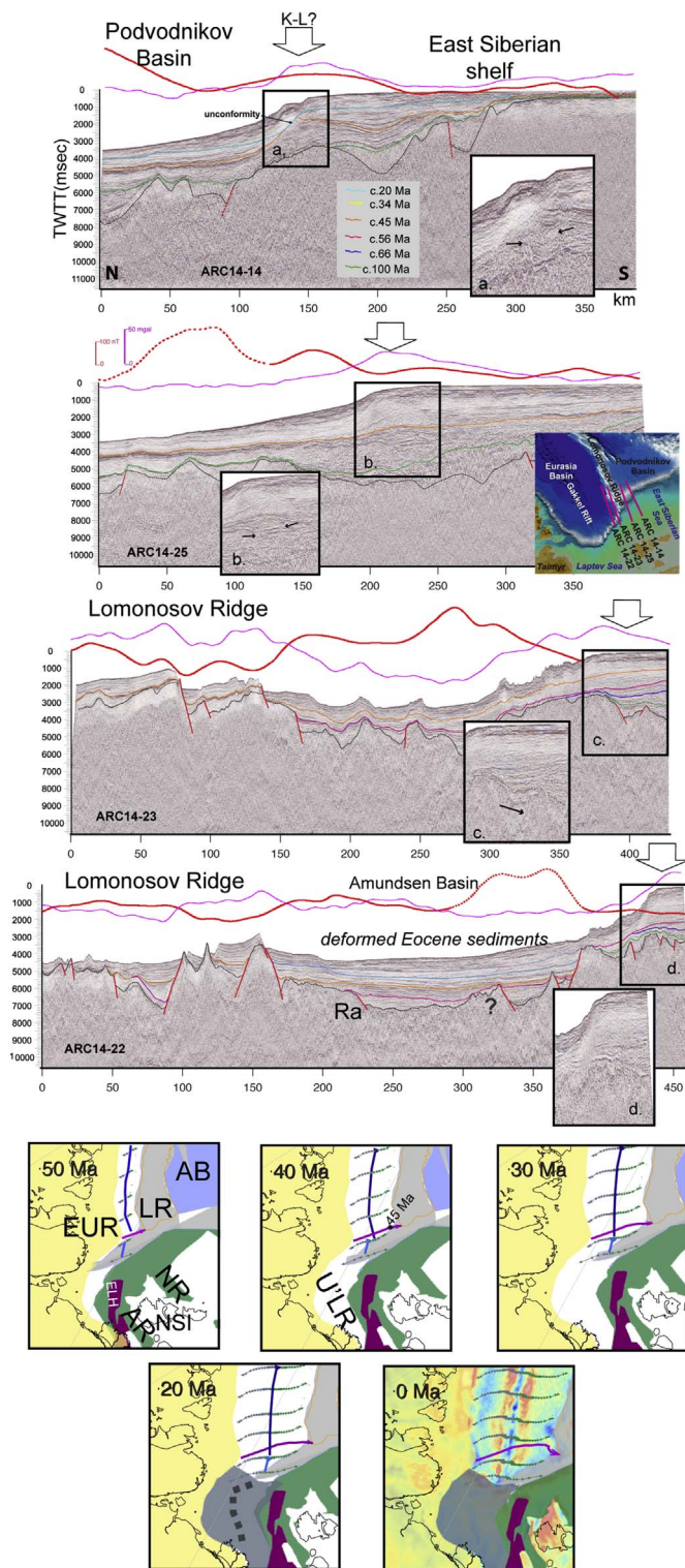
Fig. 16. Seismic lines inspected for Khatanga-Lomonosov Fault (K-L) activity (location in inset figure and Fig. 1, un-interpreted data in Fig. S7). Potential field data and bathymetric profiles as in Fig. 5. Dashed segment in the magnetic profile signals a higher data uncertainty. Lower panels show plate reconstructions of Lomonosov Ridge and adjacent regions (North American plate) relative to a fixed Eurasia (EUR) plate. Abbreviations: AB-Amerasia Basin, AR-Anisin Rift, ELH-East Laptev High, NR-Novosibirsk Rift, NSI-New Siberian Islands, U'LR-Ust'Lena Rift. Blue line is the inferred plate boundary through the Eurasia Basin, light blue line – the inferred continuation of this boundary through northern Laptev Sea, and dashed line is the inferred Oligocene-Miocene intra-continental plate boundary through the Laptev Sea. Magenta line segments show the predicted motion of Lomonosov Ridge (North American plate) relative to Eurasian plate from 55 Ma to Present in 5 myr interval. (For interpretation of the references to colour in this figure legend, the reader is referred to the web version of this article.)
