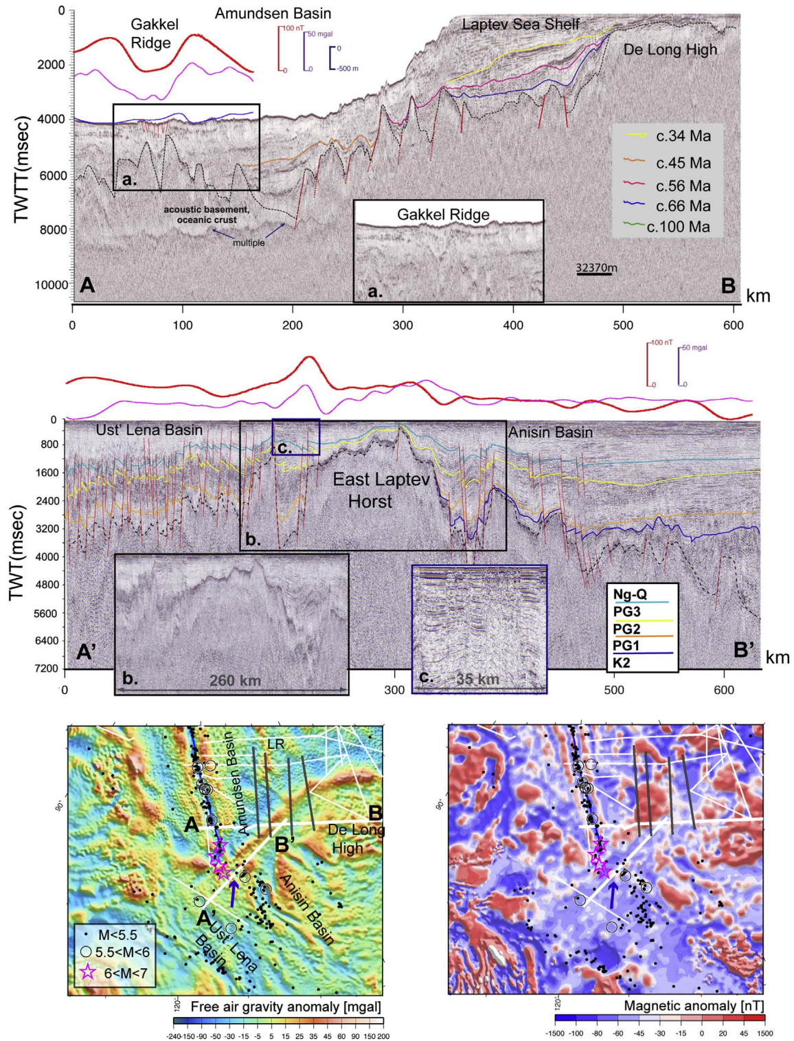
Fig. 15. Seismic lines across the easternmost end of Gakkel Ridge (AB profile: ARC2012-16), and the northernmost part of the Laptev Sea (A'B' profile: ION-11-4600) (location in inset figure and Fig. 1, un-interpreted data in Fig. S6). Lower panels show gravity anomaly (left), and magnetic gridded data (right) as in Fig. 2. Open circles, stars and dots are seismic events from ISC + EMSC earthquake catalogues from 1960 to 2016. Blue arrow indicates the small transform fault that links Gakkel Ridge to the active intra-continental plate boundary in the Laptev Sea.
