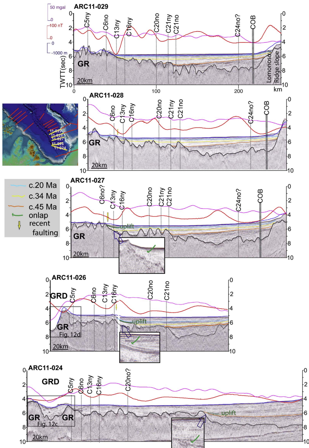
Fig. 9. Arktika-2011 (south Amundsen Basin) seismic profile interpretation (location in inset figure and Fig. 1, un-interpreted data in Fig. S4). GR stands for Gakkel Ridge, GRD is the Gakkel Ridge Deep, see sections 4.5 and 4.6. Potential field data, bathymetric profiles, and chron interpretations as in Fig. 5.
